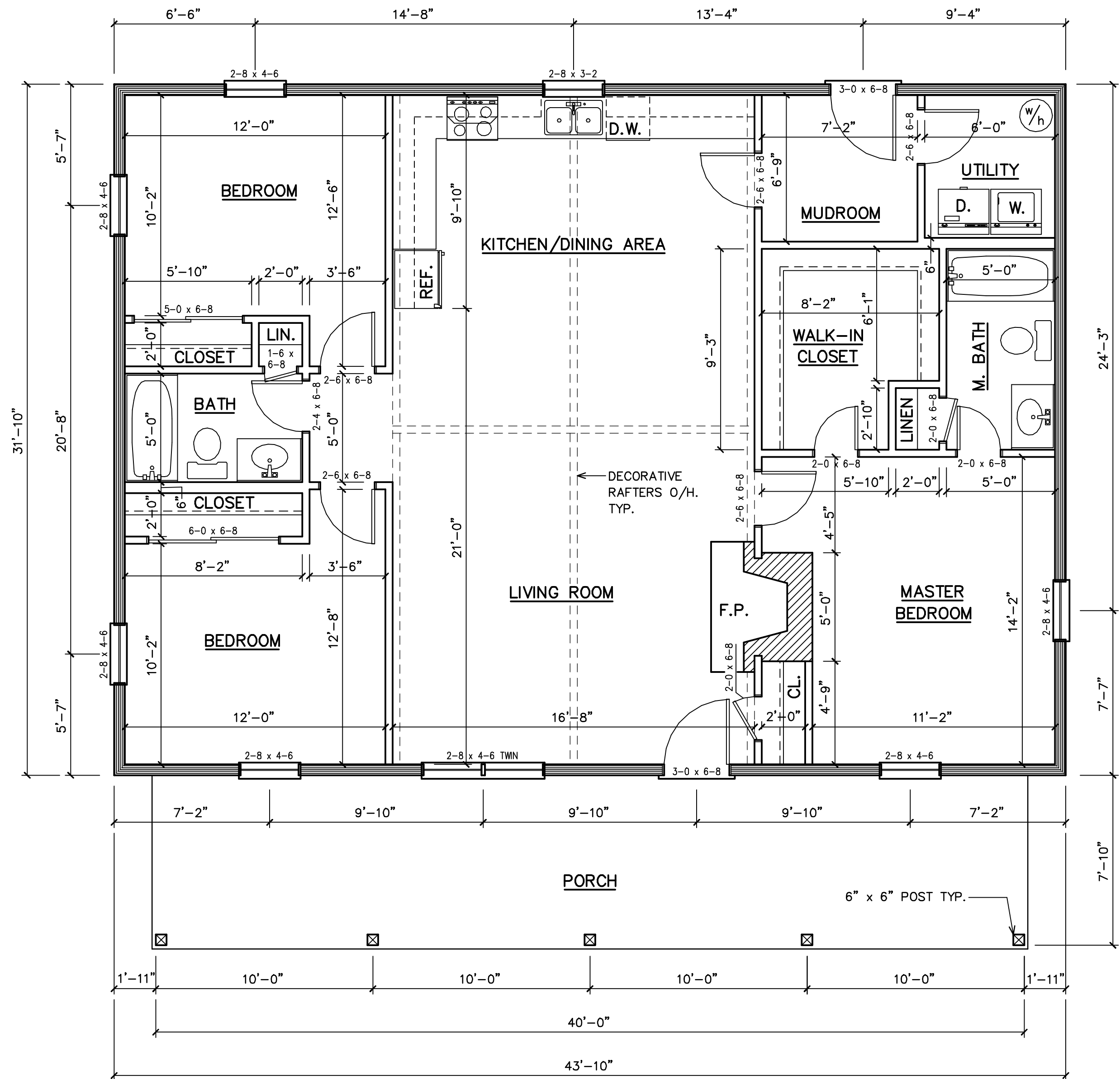
FLOOR PLAN
